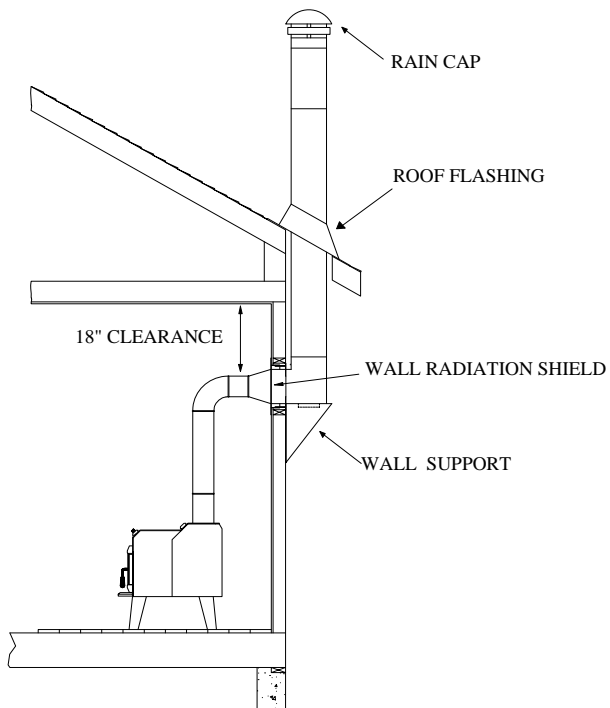
Wall installation
