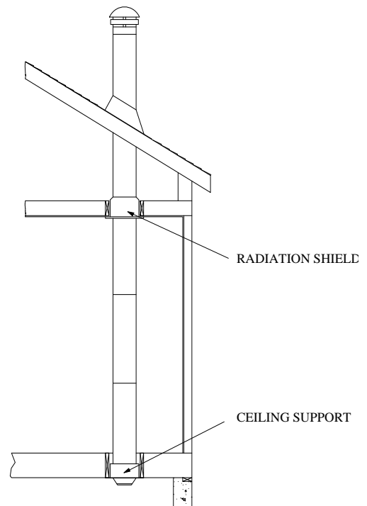
Vertical installation
